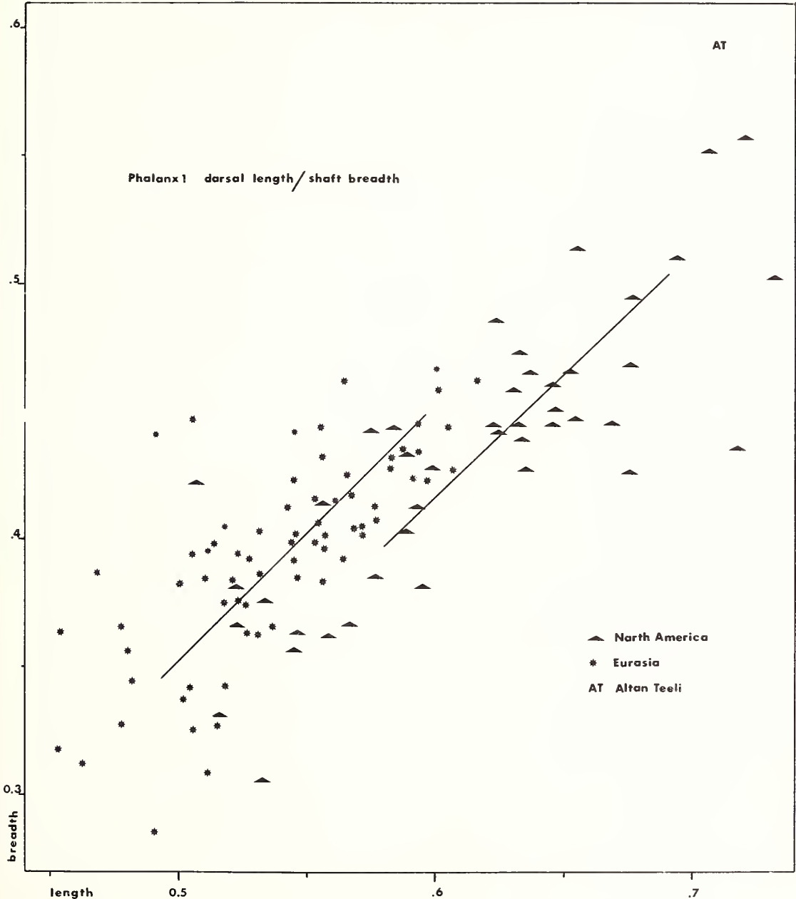
TEXT-FIG. 5. Phalanx 1 mid-shaft breadth plotted against dorsal length in Eurasian and North American Anchitherium and Hypohippus . Reduced major axis fitted to the data. AT = Sinohippus from Altan Teeli. Log data.
